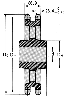
Double sprocket with hub on one side (Double C type)
