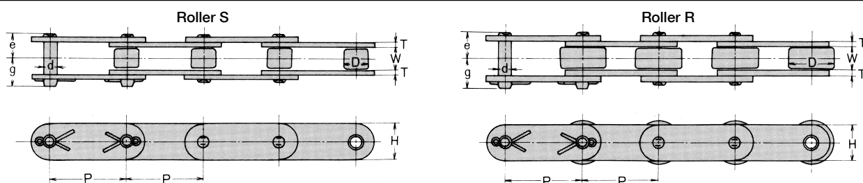
This figure shows CJ type connecting links, but RJ type connecting links are used for DID 2060 or smaller.
