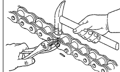
Spring pin installation method for HI-PWR-S series
