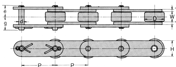
This figure shows a CJ type connecting link but R connecting links RJ type are used for DID 2060 or smaller.
